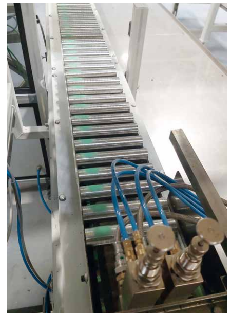
Discharge conveyor belt with optional marking station for OK/NOK.
